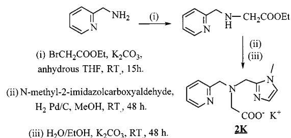
Scheme 1. IPGK ( 2K ) synthesis
