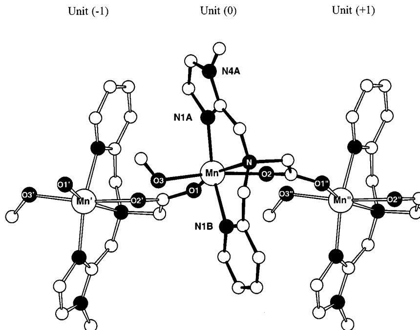
Figure 1. ORTEP drawing of complex 3 cationic chain with three adjacent monomeric units of the polymer; hydrogen atoms have been omitted for clarity
