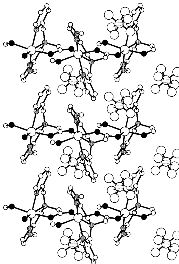
Figure 3. ORTEP packing diagram; the disorder of the anionic units has been omitted for clarity
